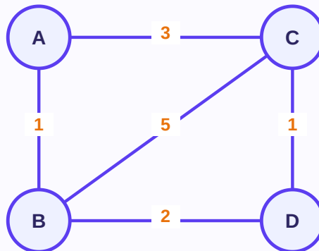
Weighted Graph
