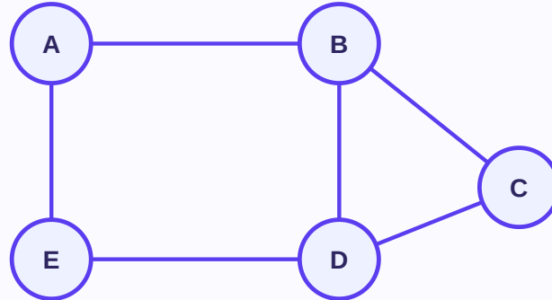
Undirected Graph
